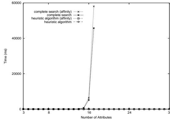
Fig. 13. Computational time of the algorithms
