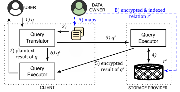
Fig. 2: Query execution process
